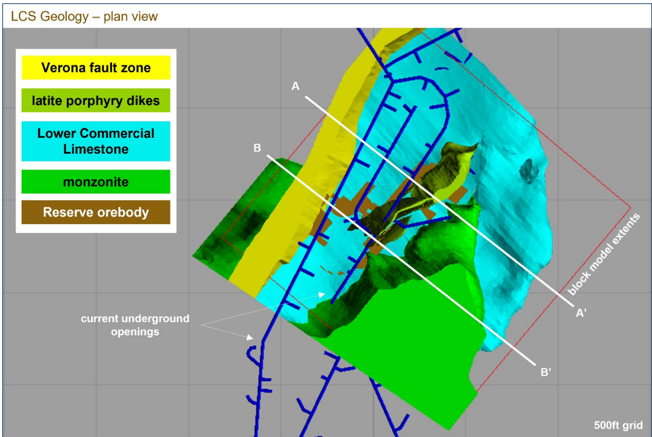
Figure 3 LCS Geology
